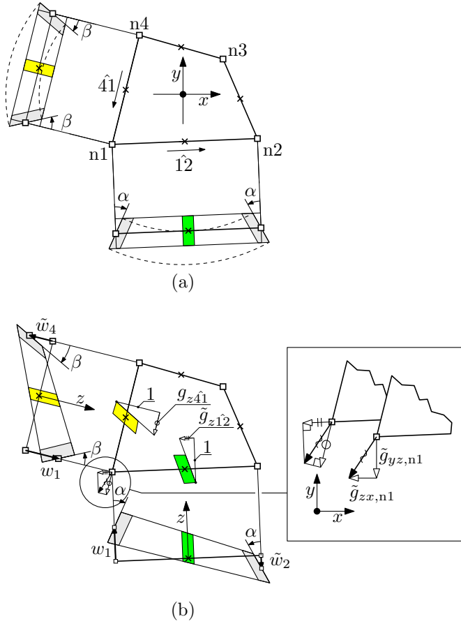
Figure 2.13: A transverse shear sampling technique employed in the four-noded isoparametric element for preventing shear locking in the oop plate bending.
