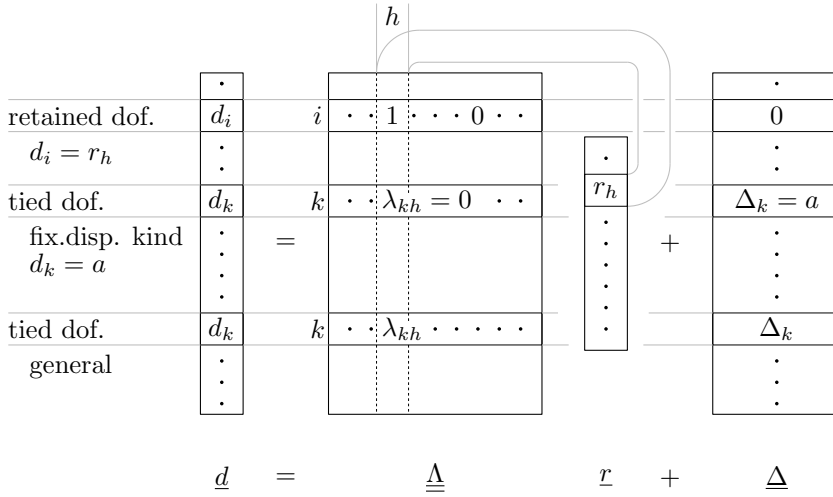
Figure 2.20: Graphical representation for the \underline{\Lambda} matrix and for the \underline{\Delta} vector in Eq. 2.136; representative matrix rows are illustrated for a retained dof, and for two tied dofs, namely a fixed displacement subcase, and the general case.
