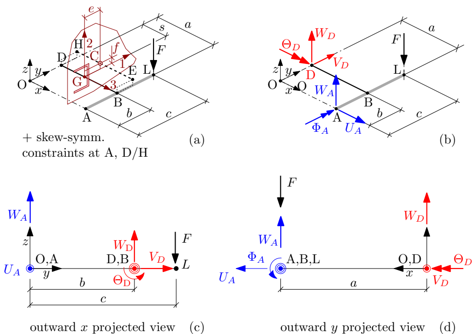
Figure 1.28: A quarter portion of the ladder frame, which is the minimal portion to be modeled due to the dual skew-symmetry. Please note that the (O,xyz) reference system of the present figure coincides with its fixed counterpart as in Fig. 1.27 in the undeformed configuration only. The present figure reference frame partly follows, in fact, the structure deflection.
