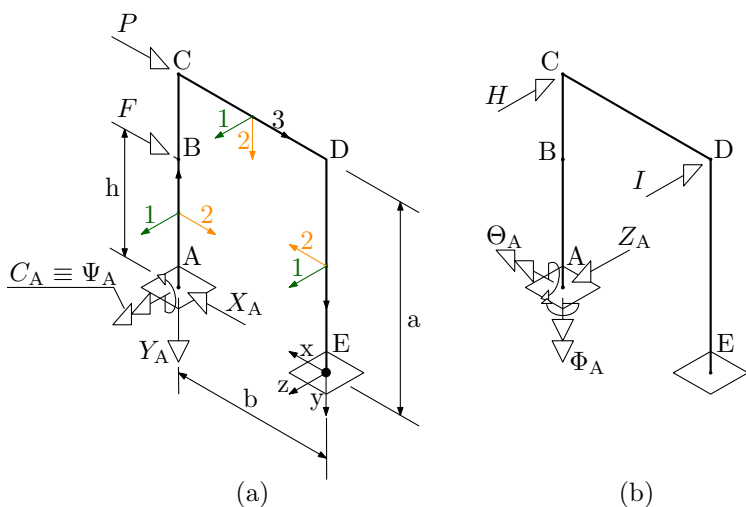
Figure 1.24: A rollbar-like frame; Figures a) and b) collect the considered in-plane and out-of-plane actions, respectively, which are split for added readability.
