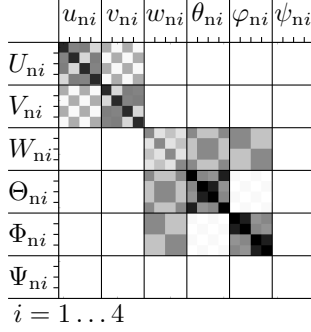
Figure 2.15: A representation of the stiffness matrix terms for each element in the example structure; the term magnitude is represented through a linear grayscale, spanning from zero (white) to the peak value (black).
