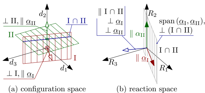
Figure 2.19: Allowed system configurations and constraint reactions for the pedagogical example of Fig. 2.18. The allowed virtual displacement sets are easily derived as the homogenous counterpart of (a), and are left to the reader's imagination.
