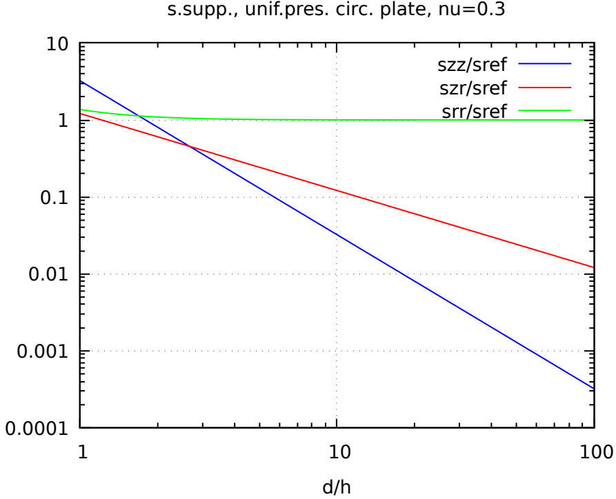
Figure 2.2: Normalized stress component magnitude in the case of a simply supported circular plate subject to normal pressure, according to the spatial theory of elasticity framework, see [?, p.349]. A homogeneous and isotropically elastic circular plate of diameter d and thickness h is simply supported along its perimeter (i.e. apart from the their transverse component, displacements are free, and so are rotations), and it is loaded by a unit pressure at its upper surface. The peak magnitude of the transverse stress \sigma_z is observed at the pressurized surface, and it equates the pressure value. The oop shear stress \tau_{zr} is maximal along the perimeter, and it equates \frac{3}{8} \left(\frac{d}{h}\right) . The two ip direct stress components \sigma_r, \sigma_\theta reach a common the peak value of \frac{3(\nu+3)}{32} \left(\frac{d}{h}\right)^2 + \frac{\nu+2}{20} in correspondence of the plate center, at the stretched surface; its thin plate counterpart, \sigma_{\text{ref}} = \frac{3(\nu+3)}{32} \left(\frac{d}{h}\right)^2 , lacking of the O\left(\left(\frac{d}{h}\right)^0\right) , is taken as the normalizing stress value. The remaining \tau_{r\theta}, \tau_{\theta z} stress components are zero due to axisymmetry. The commonwise \nu = 0.3 Poisson ratio value is used in tracing the Figure.
